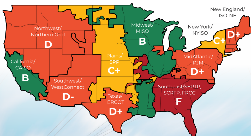
FIGURE 1 Overall regional transmission planning grades
